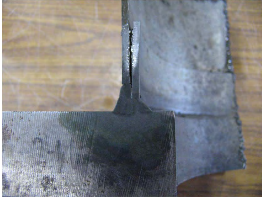
Figure 3.2: Cross Section of a Typical Full Penetration Connection
