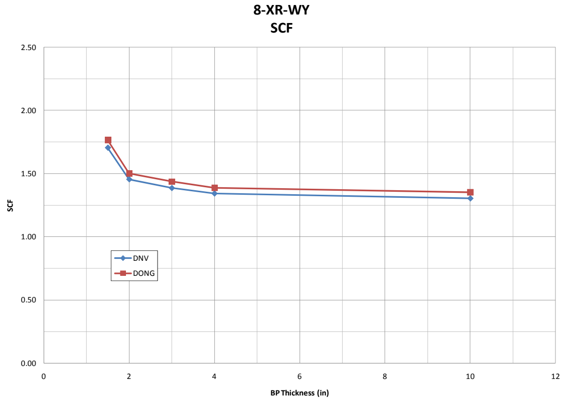
Figure 4.2: 8-XR-WY (SCF versus Base Plate Thickness)
