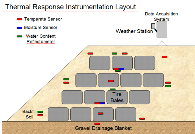
Figure 4.2: Instrumentation Profile for the Thermal Response of the Tire Bale Slope
