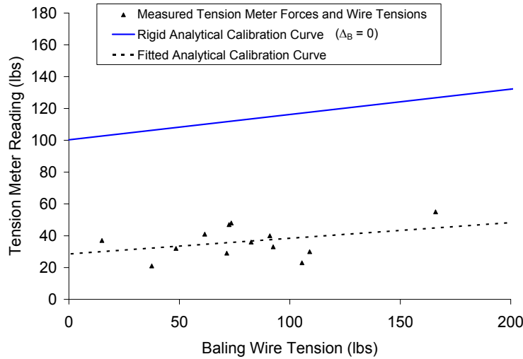
Figure 3.3: Tension Meter Forces and Wire Tensions for the Passenger Vehicle Cylinder Bales
