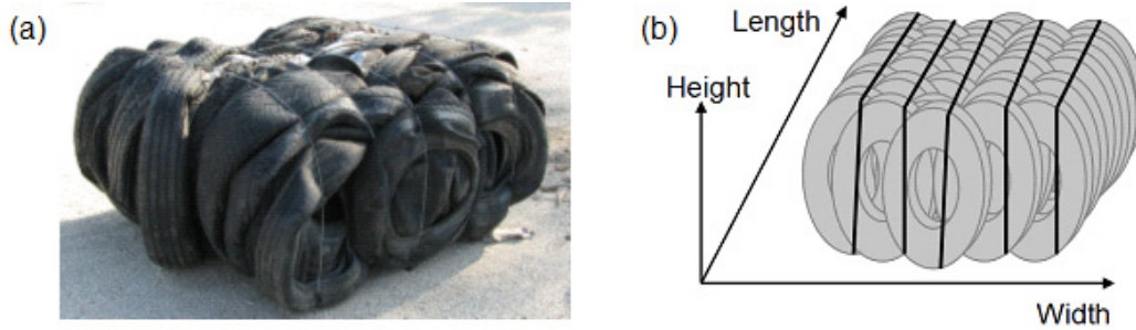
Figure 2.7: (a) Photograph of a Block Tire Bale and (b) Illustration of the Block Bale Dimensions
