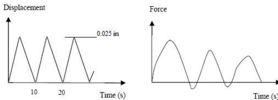
Figure 3.7: OT Load Scheme
