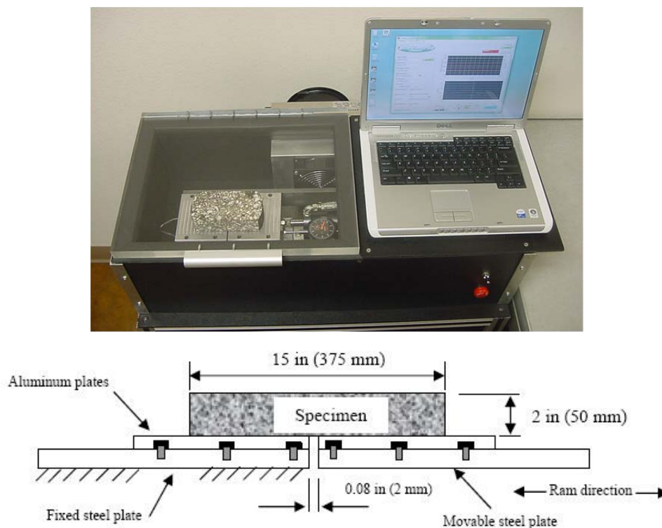
Figure 3.6: OT Apparatus
